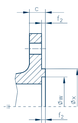
Form/Type C Feder
