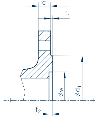
Form/Type G O-Ring-Vorsprung
