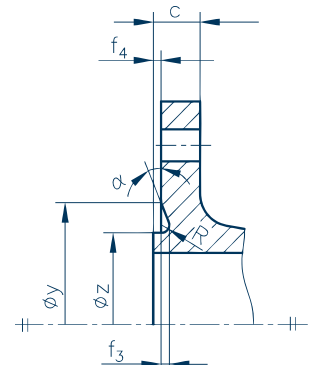
Form/Type H O-Ring-Nut
