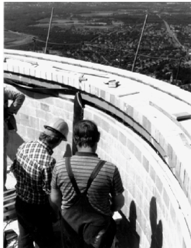
Technicians installing a lining joint sealing.
