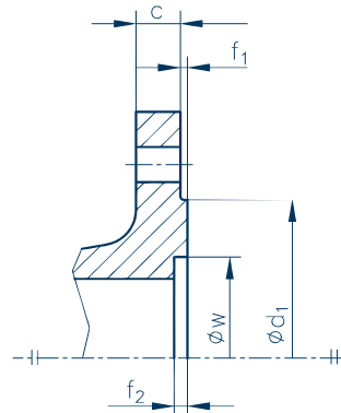
Form/Type G O-ring spigot
