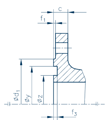
Form/Type D Groove
