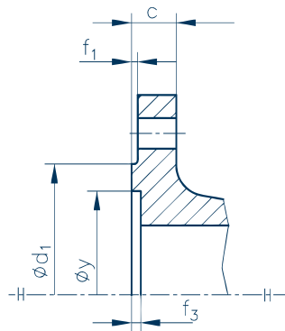
Form/Type F Recess (female Face)
