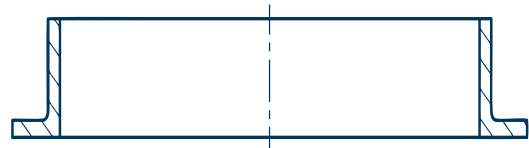
Typ 36 pressed collar with long neck
