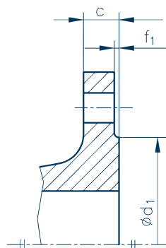
Form/Type B Raised face (B1 and B2)*
