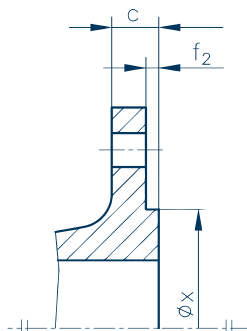
Form/Type E Spigot (male Face)
