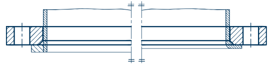
Typ 02 Loose plate flange with weld-on collar type 32 or lapped pipe end type 33
