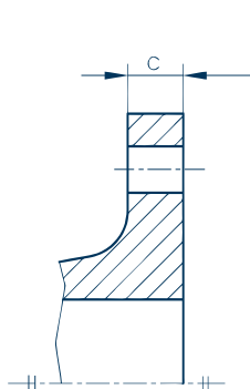
Form/Type A Flat face
