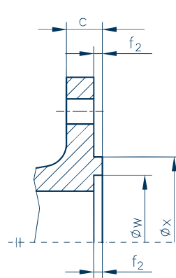
Form/Type C Tongue
