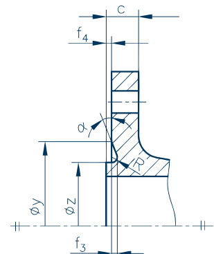
Form/Type H O-ring groove
